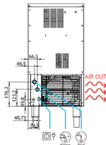
REAR VIEW VISTA TRASERA
